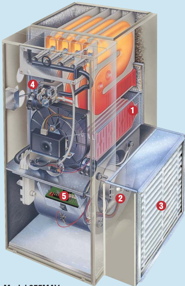
Model 355MAV shown with optional Bryant High Efficiency Media Filter.
